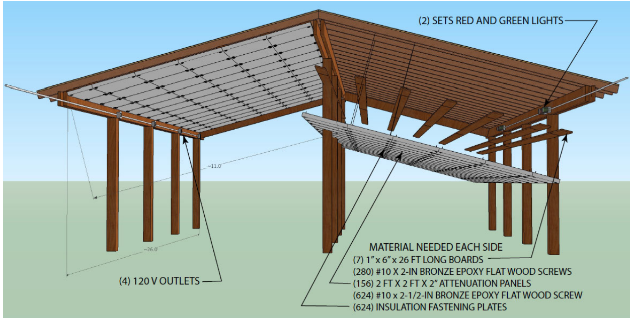
Figure 3 — 4 Bay Approximate Dimension Exploded View
