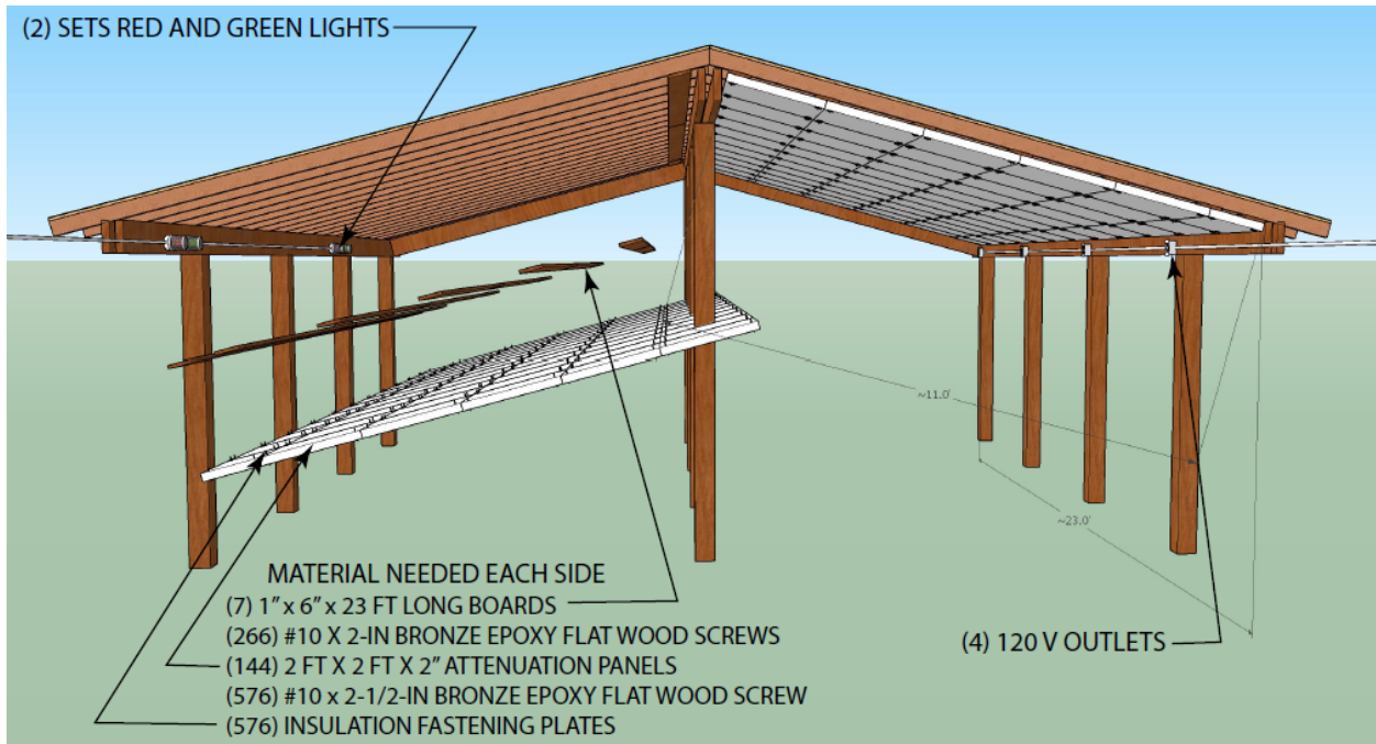
Figure 4 — 3 Bay Approximate Dimension Exploded View
